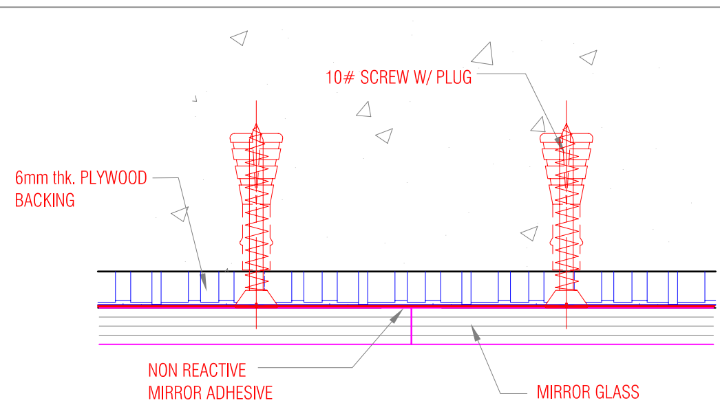
DETAIL-2
