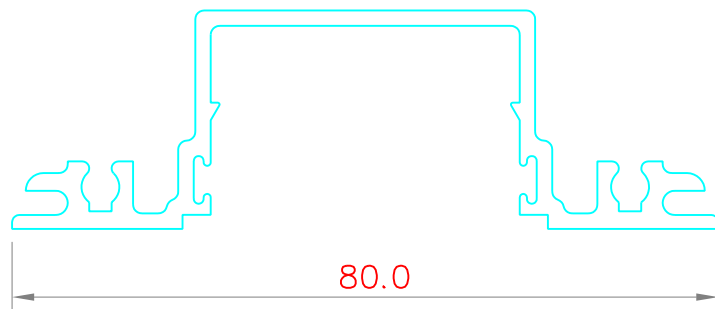
GLAZING ADAPTOR
