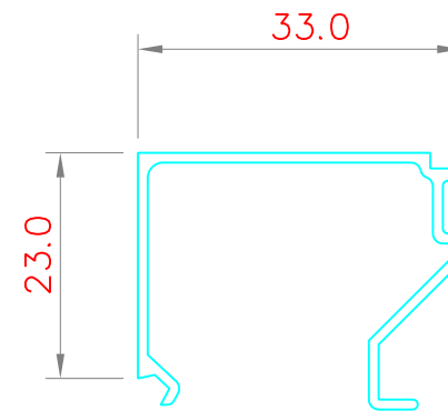
GLAZING BEAD
