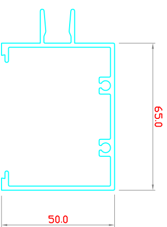
HEAD / SILL / TRANSOM FRAME 5000-SP10
