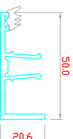
HEAD / SILL OR TRANSOM CAP (OPERABLE WINDOWS) 5000-SP17
