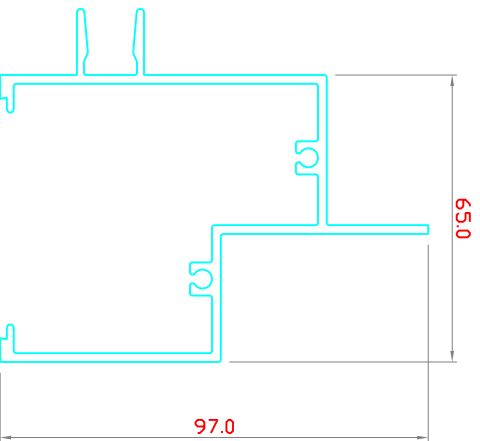
HEAD / SILL / TRANSOM FRAME w / AWNING RETAINER 5000-SP11
