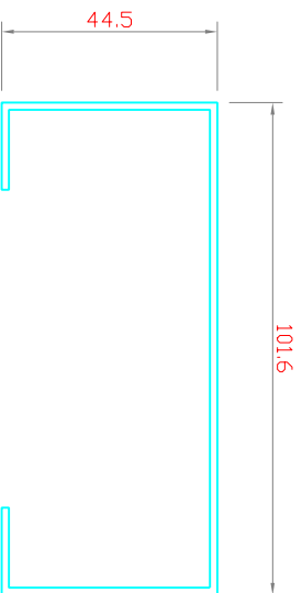
101.6 x 44.5 OPEN BACK FRAME
