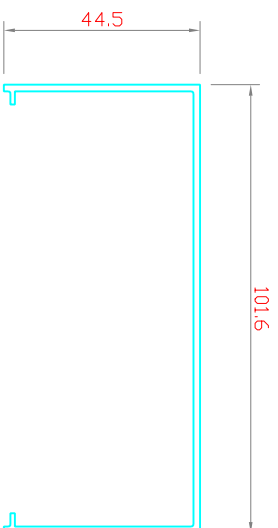
101.6 x 44.5 SPLIT TUBE FRAME
