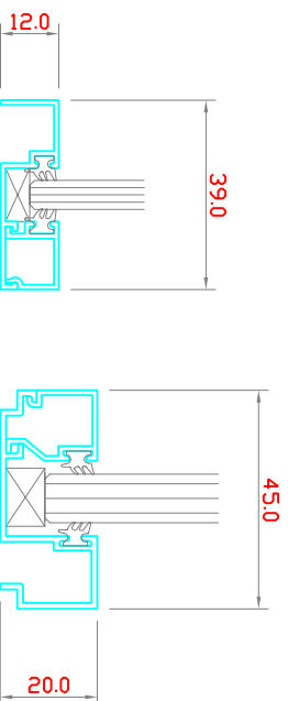
SNAP ON BASE 6mm GLASS SNAP ON BASE 8.0 TO 12.0mm GLASS
