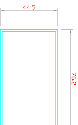
76.2 x 44.5 RECTANGULAR TUBE
